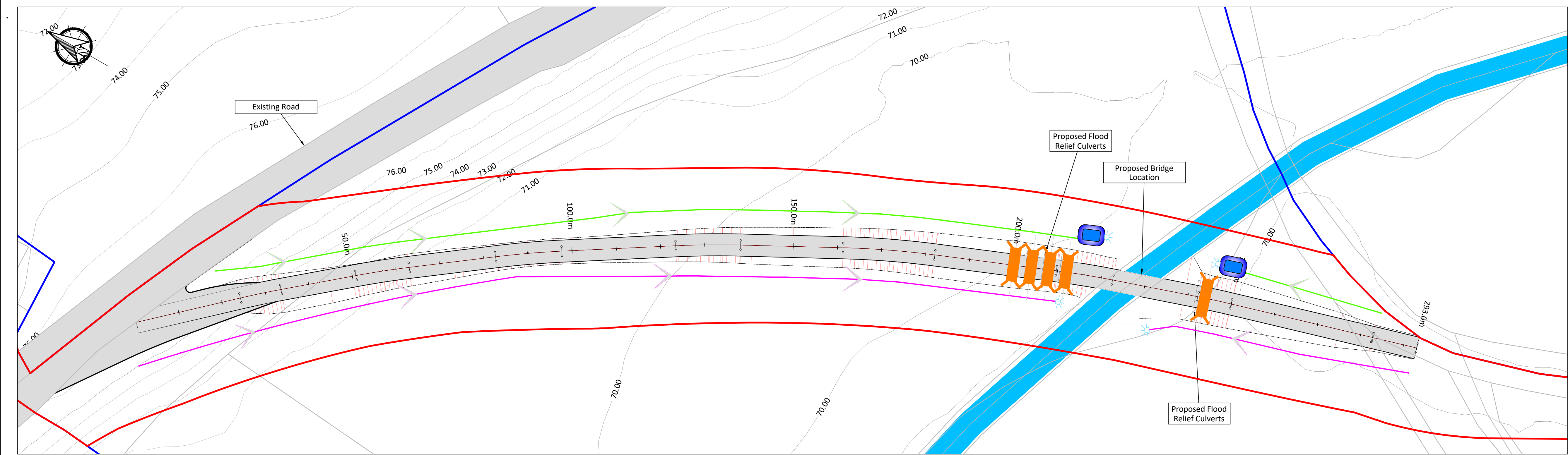
PLAN Scale 1:500
